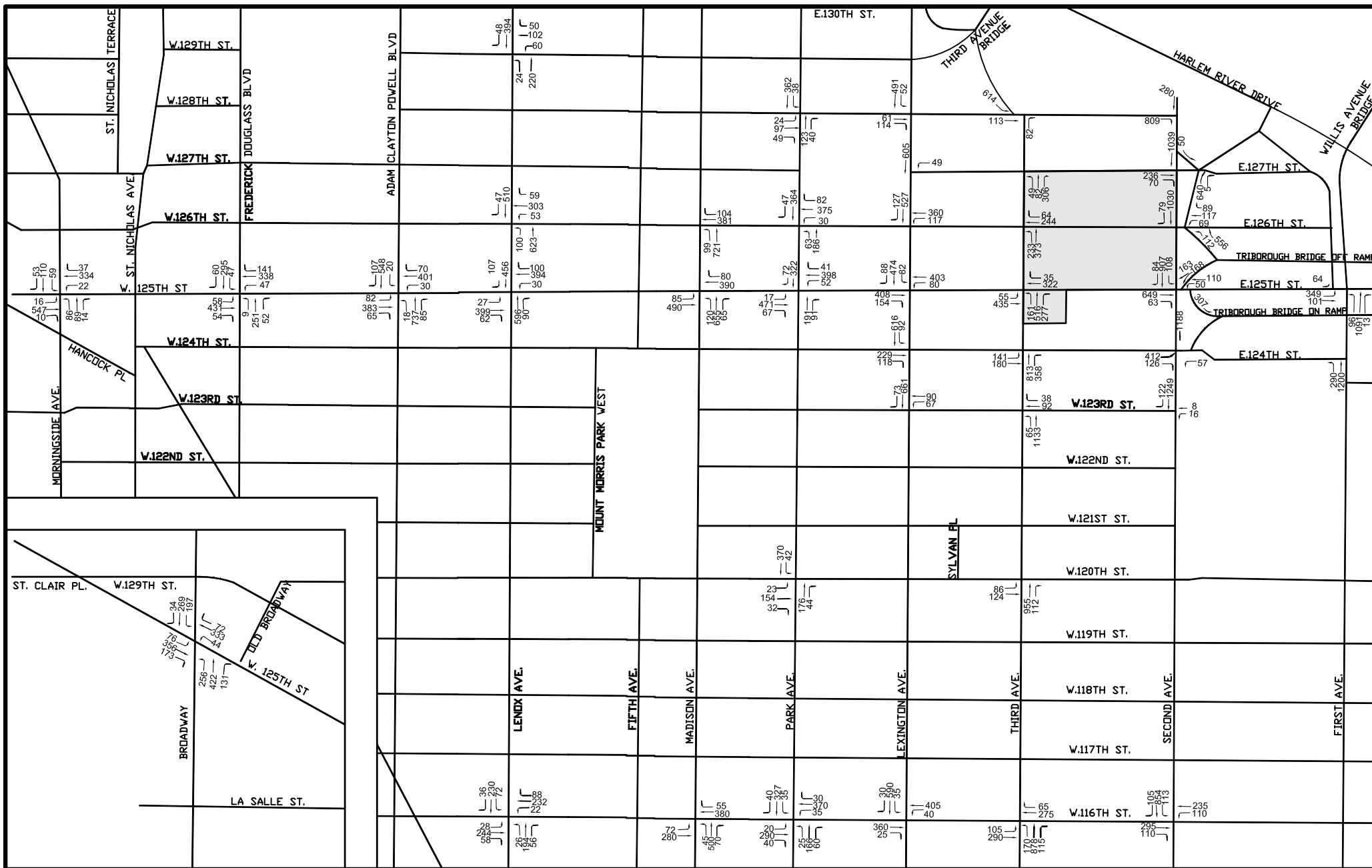
Figure 3.15-4 2007 Existing Weekday MD Peak Hour Traffic Volumes
